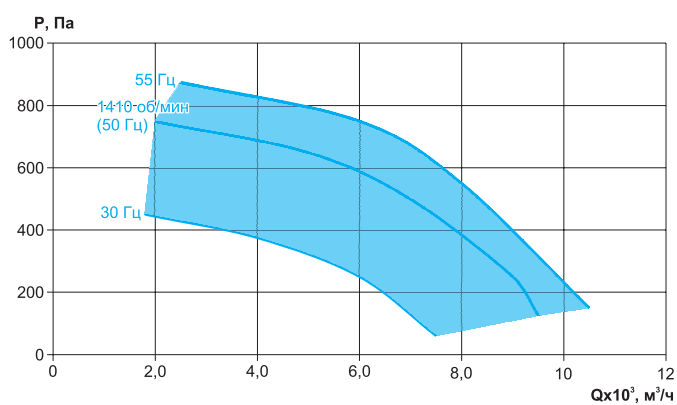
VCN-80-50/50-Ex1/IIIB-ПЦ-2,2/1500/220-380
