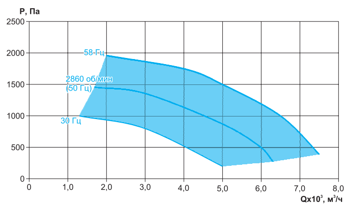
VCN-60-35/35-Ex1/IIIB-ПЦ-3,0/3000/220-380
